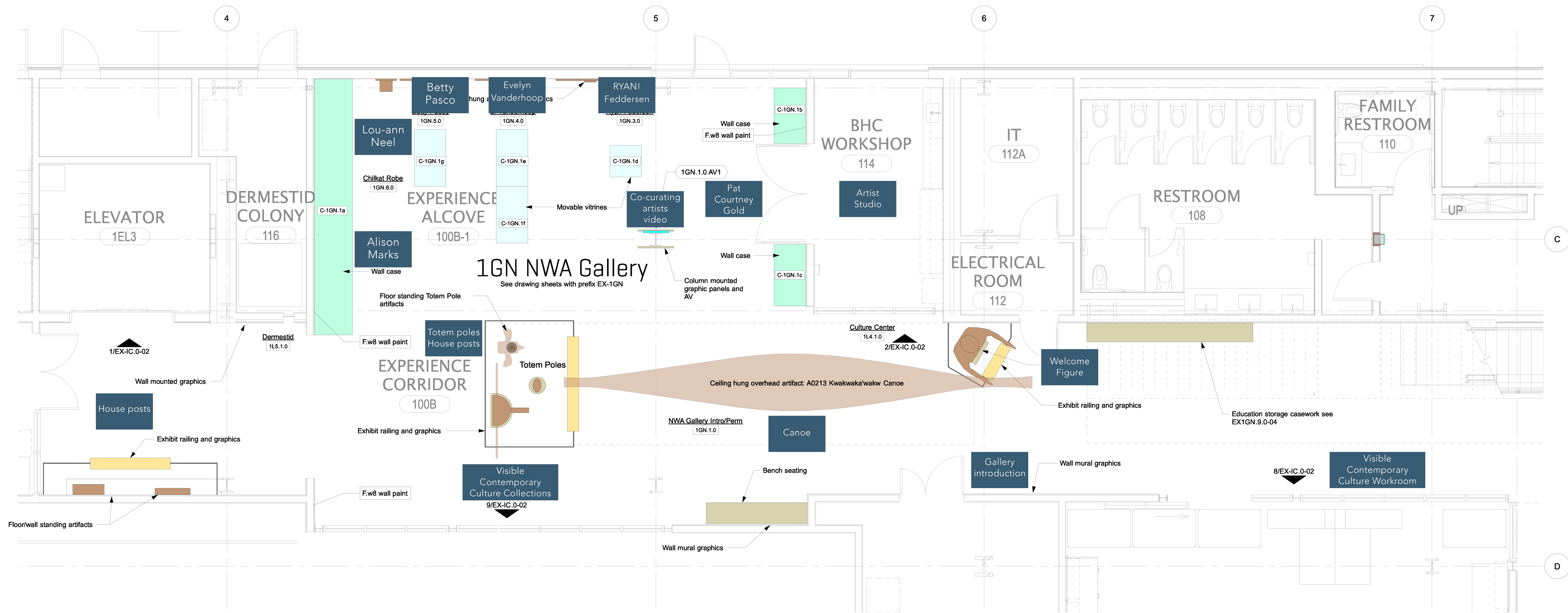
1 1GN NWA Gallery Exhibit Plan Scale: 1/4" = 1'-0"
