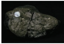
Brecciated bomb
